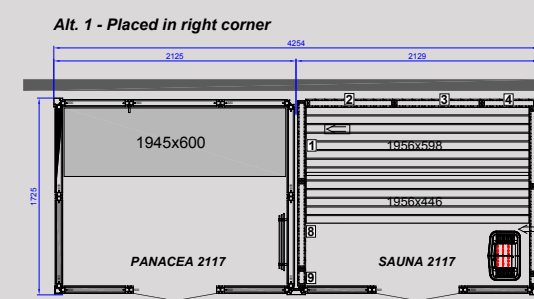
TWIN PANACEA 2117 Size: D 1725 x W 4254 mm
