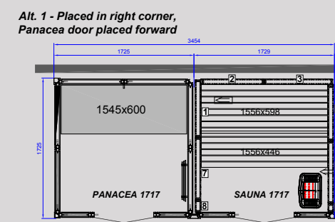
TWIN PANACEA 1717 Size: D 1725 x W 3454 mm
