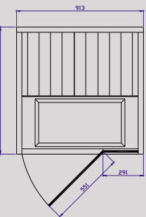
TYLÖSAND T-810 Size: D 913 x W 913 mm
